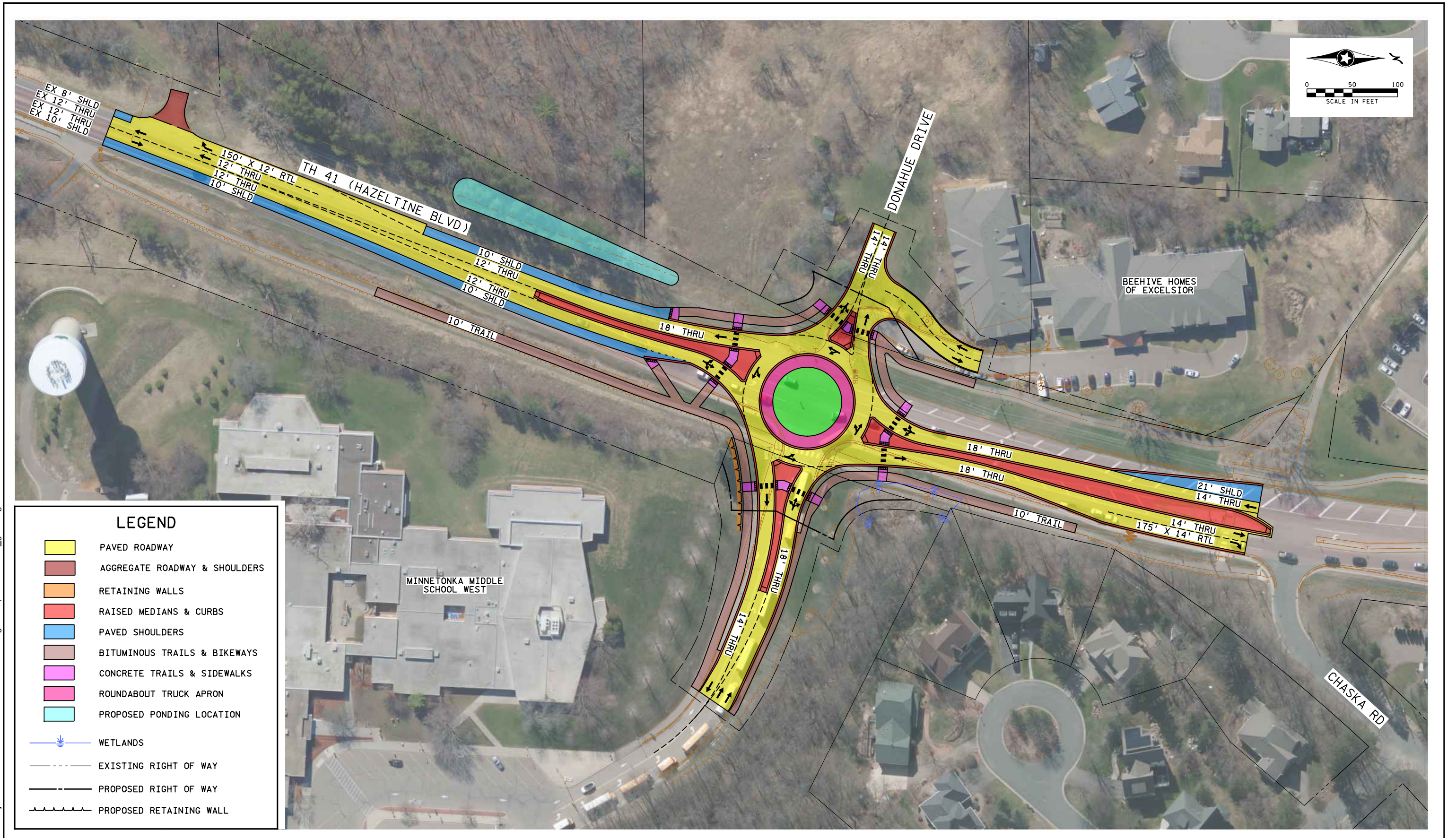
TH 41 and Minnetonka Middle School West Concept Graphic Proposed Roundabout City of Chanhassen
